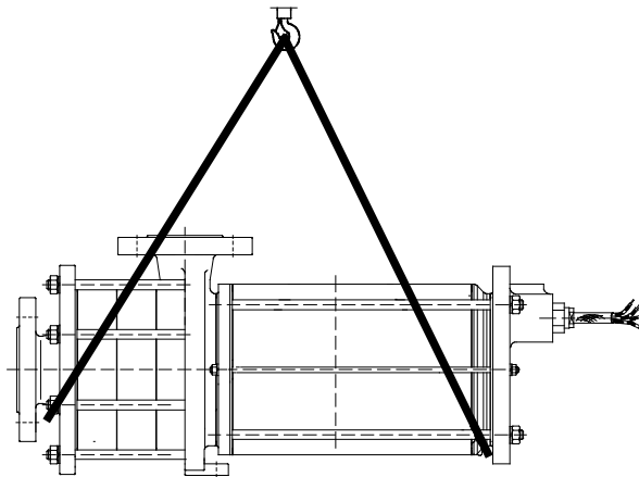
Abb. 5: Hebezeug befestigen an Pumpenaggregat
